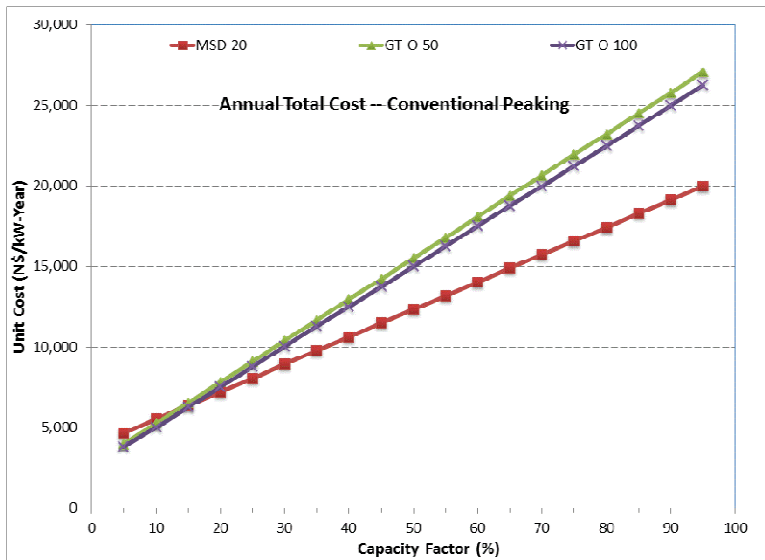
Figure 6-4: Total annual Costs of Conventional Peaking Plants
