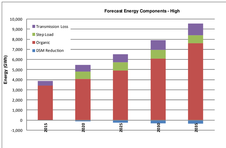
Figure 5-14 – High Forecast Components (GWh)
