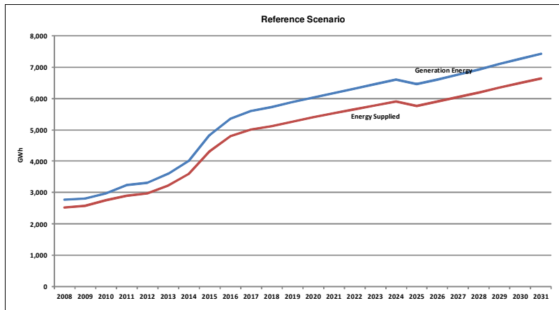
Figure 5-1 – Reference Sales and Generation (GWh)
