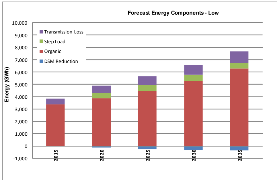
Figure 5-11 – Low Forecast Components (GWh)
