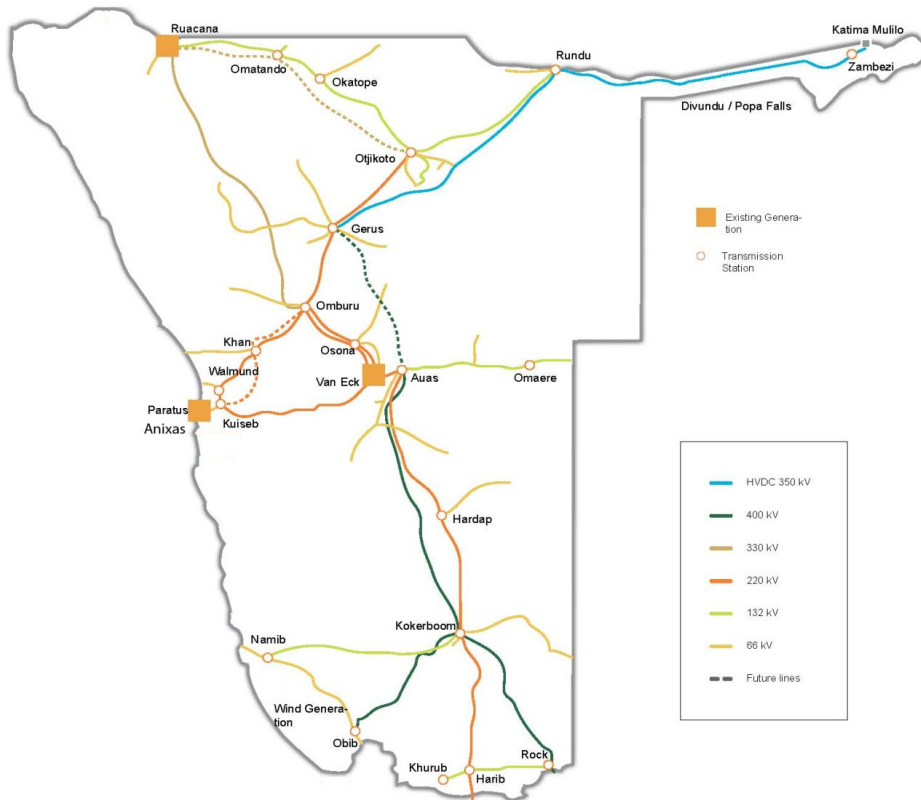
Figure 2-3: Transmission System of Namibia
