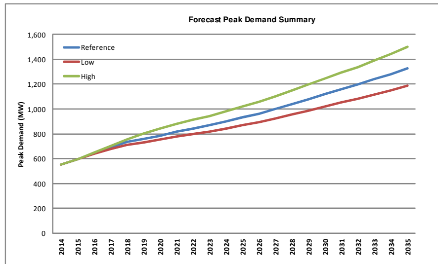
Figure 5-6 – Overall Generation Forecasts – Peak Demand (MW)
