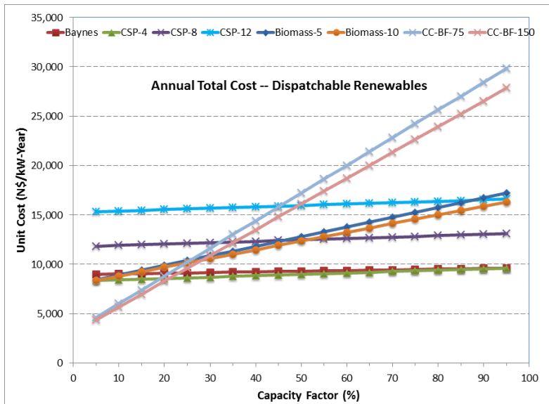
Figure 6-6: Total Annual Costs of Dispatchable Renewable Resources
